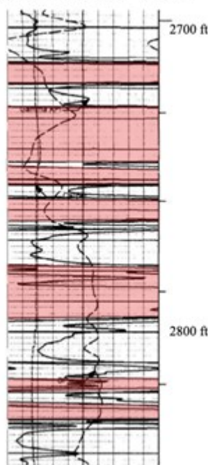
Figure 1: Samson Powerline 12-1 Logs Indicating High Gamma Ray Anomalies
